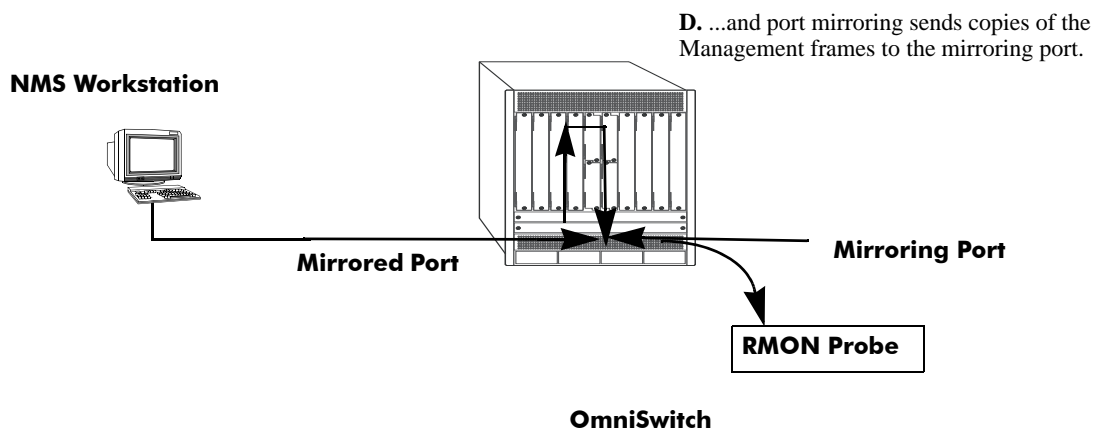
Port Mirroring Using External RMON Probe
